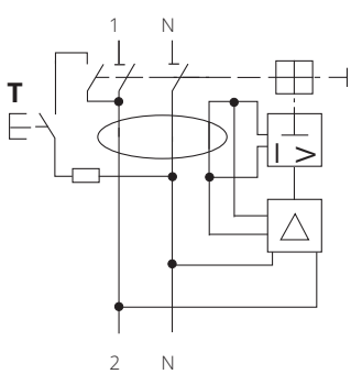
NF12BK
