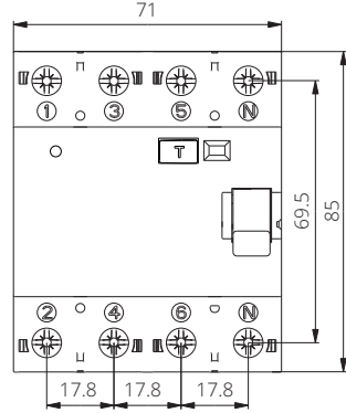
FI4BK FI4BS
