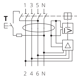
FI4BK, FI4BS
