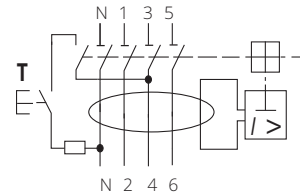
FI4-L, FI4K-L, FI4S-L, FI4F-L
